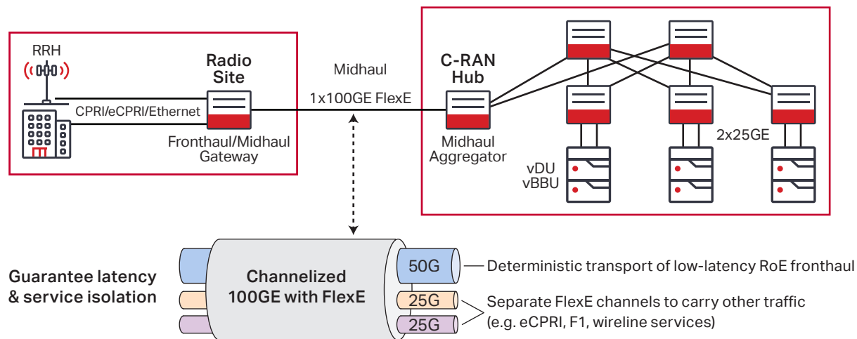
Figure 4. 5164 Channelized FlexE
