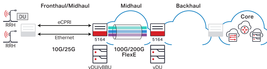
Figure 1. Cloud-RAN network application
