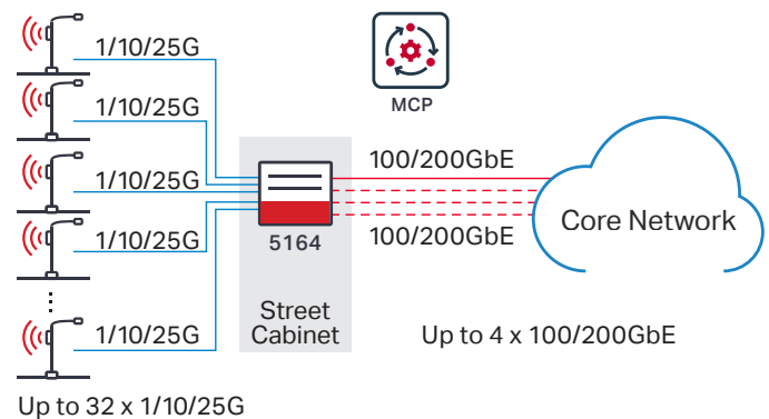
Figure 3. 5164 Router outside service and aggregation
