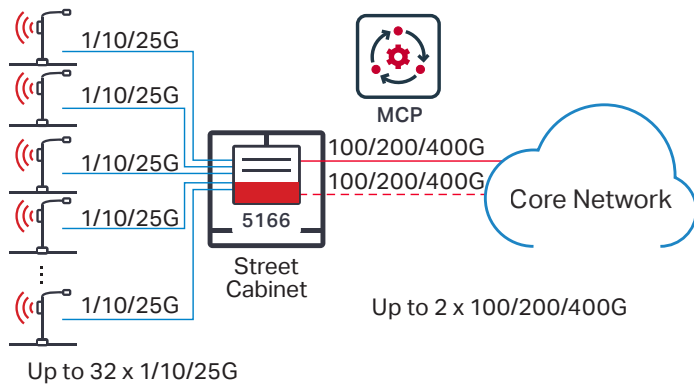
Figure 3. 5166 Router outside service and aggregation
