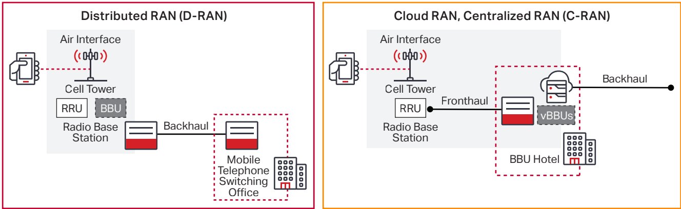
Figure 2. 5G NR RAN architecture
