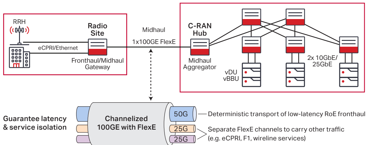
Figure 4. 5166 Channelized FlexE
